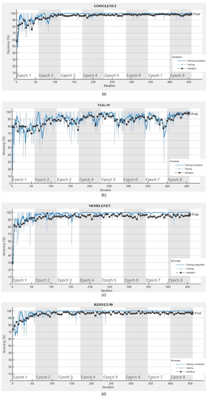
FIGURE 5 Training and verification graphs for all models: (a) GoogLeNet, (b) VGG-19, (c) MobileNet-v2, and (d) ResNet-50.
