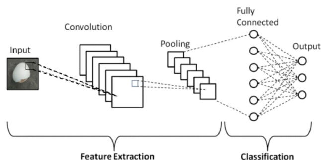
FIGURE 3 Convolutional neural networks (CNN) architecture. Source: Gurucharan (2024).
