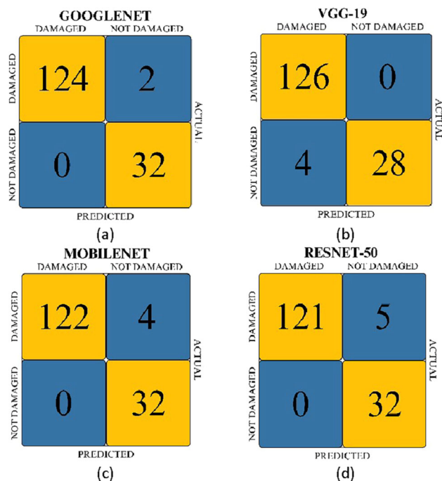
FIGURE 6 Confusion matrix results for all models (a) GoogLeNet, (b) VGG-19, (c) MobileNet-v2, and (d) ResNet-50.
